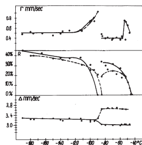
Fig. 2. Temperature dependence of Mössbauer effect intensity R , line width \Gamma and quadrupole splitting \Delta for \text{Fe}(\text{ClO}_4)_2 (• full line) and \text{FeCl}_2 (○ dashed line) solutions.
