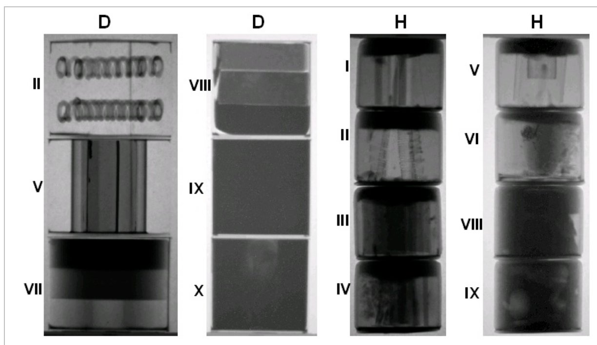
Figure 2 - Neutron radiographs of selected black boxes measured at ANTARES
