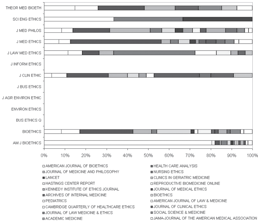
Figure 1. Comparative analysis of citation patterns.
