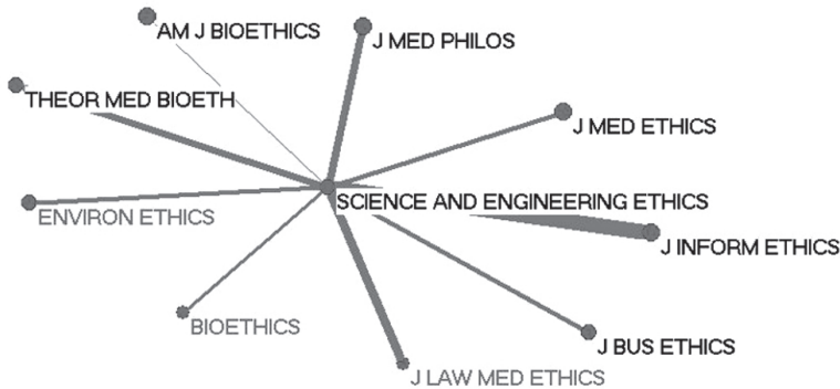
Figure 2. Selective Co-citation pattern for SCI ENG ETHICS. Similarity measure: S_{ij} = \frac{C_{ij}}{C_i C_j}
