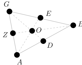
Figure 4. The centroid of a triangle always exists.
