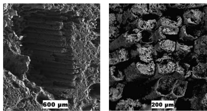
Fig 8. Secondary electron image on remnants of sawdust grain. On the left image, totally preserved fibers from the structure of wood. On the right, detailed image of fibers
