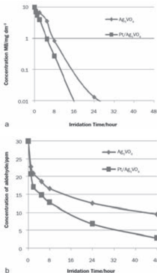
Fig. 5. Photocatalytic performance of silica gel beads coated with Ag 3 VO 4 and Pt loaded Ag 3 VO 4 , respectively in fluorescent light (a) decomposition of methylene blue and (b) decomposition of acetaldehyde
