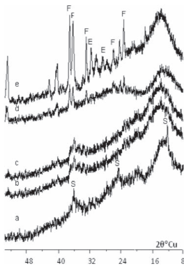
Fig. 4. The X-ray powder diffraction patterns of the SJ-2 heat-treated at the temperatures: a – 600 °C; b – 650 °C; c – 700 °C; d – 750 °C; e – 850 °C. S – serpentine; F – forsterite; E – enstatite
