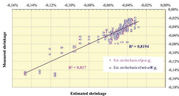
Fig. 18. Deformation of the prisms with CEM III/B 32.5 N-S at days 28, 56 and 112, comparing the values estimated using Eqs. (35) and (36) and the values actually measured, during the ÉMI experiments of 2010.
