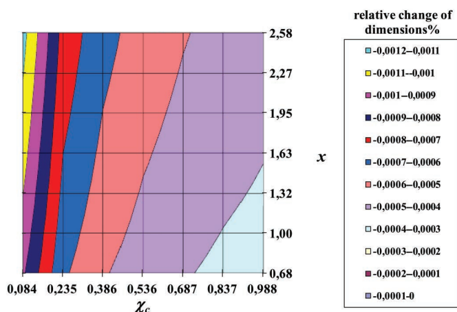
Fig. 19. Nomogram of deformation estimates based on x-\chi_c-p/a for mixes made with CEM III/B 32.5 N-S at the age of t=112 days, when p=0.294 and f/f_a=183 (medium sand content aggregate)
