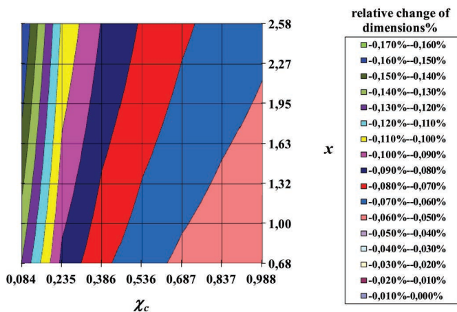
Fig. 21. Nomogram of deformation estimates based on x-\chi_c-p/a for mixes with CEM III/B 32.5 N-S at the age of t=112 days, when p=0.294 and f/f_a=119 (medium sand content aggregate)
