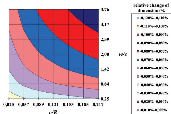
Fig. 20. Nomogram of deformation estimates based on w/c-c/R-\chi_c for mixes made with CEM III/B 32.5 N-S at the age of t=112 days, when \chi_c=0.99 and f/f_a=183 (neat cement paste powder, medium sand content aggregate)
