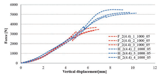
Fig. 10. Force vs. vertical displacement of laminated glasses consisted of 2×4 mm HSG or float glass layers with height of 1000 mm
