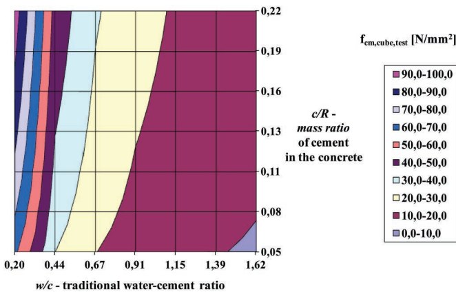
Fig. 14. w/c - c/R -(1- l )-based nomogram for mixes with stone powder and CEM III/B 32.5 N-S, based on experiments at ÉMI in 2010, ( l = 0.010 )
