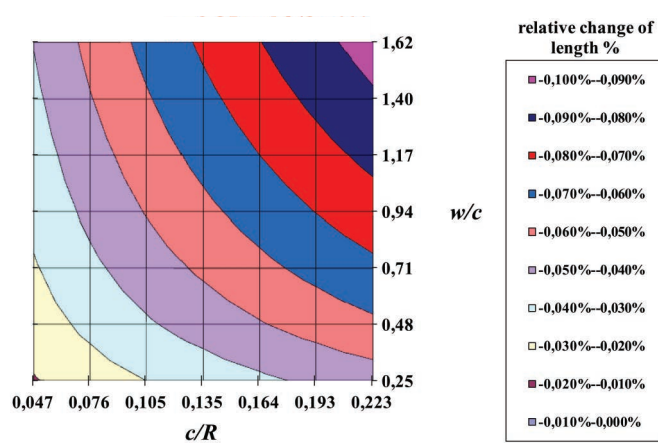
Fig. 26. Nomogram of deformation estimates based on w/c - c/R - \chi_c for mixes with CEM I 42.5 N at the age of t=112 days, when \chi_c=0.85 and f_2/f_1=111 (15% v/v additions, high sand content aggregate)
