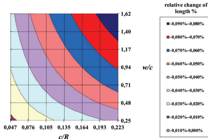
Fig. 24. Nomogram of deformation estimates based on w/c - c/R - \chi_c for mixes with CEM I 42.5 N at the age of t=112 days, when \chi_c=0.99 and f_2/f_1=186 (pure cement paste powder, medium sand content aggregate)
