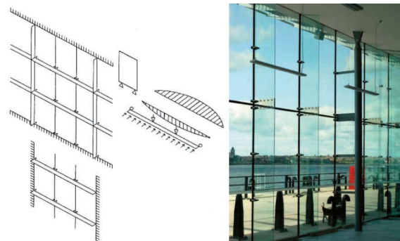
Fig. 4. Multi-storey glass columns with use of Pilkington Planar™ coupling system [1, 8]; Cruise Liner Ferry Terminal, Liverpool, UK
