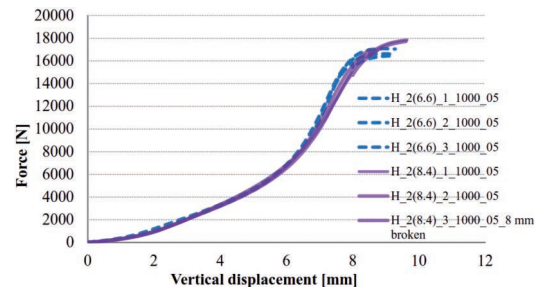
Fig. 11. Force vs. vertical displacement of laminated specimens consisted of 6+6 mm or 8+4 mm HSG glass layers with height of 1000 mm
