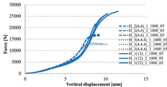
Fig. 8. Force and vertical displacement of HSG single and laminated glass specimens with total nominal thickness of 12 mm and height of 1000 mm
