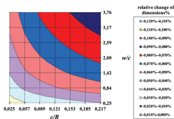
Fig. 22. Nomogram of deformation estimates based on w/c-c/R-\chi_c for mixes with CEM III/B 32.5 N-S at the age of t=112 days, when \chi_c=0.99 and f/f_a=119 (pure cement paste powder, high sand content aggregate)
