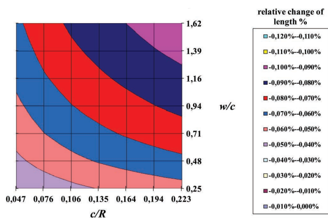
Fig. 25. Nomogram of deformation estimates based on w/c - c/R - \chi_c for mixes with CEM III/B 32.5 N-S at the age of t=112 days, when \chi_c=0.85 and f_2/f_1=119 (15% v/v additions, high sand content aggregate)
