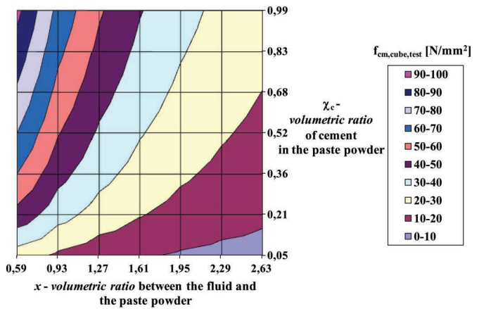
Fig. 13. x - \chi_c - p - l -based nomogram for mixes with stone powder and CEM I 42.5 N, based on experiments at ÉMI in 2010, ( p = 0.280 ; l = 0.010 )
