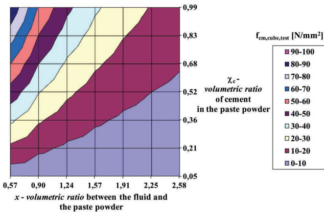
Fig. 12. x - \chi_c - p - l -based nomogram for mixes with stone powder and CEM III/B 32.5 N-S, based on experiments at ÉMI in 2010, ( p = 0.280 ; l = 0.010 )
