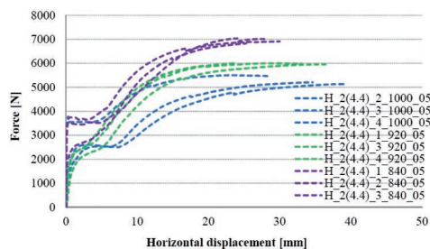
Fig. 9. Force vs. horizontal displacement of laminated glasses consisted of 2×4 mm HSG glass layers with 1000 mm, 920 mm as well as 840 mm nominal heights
