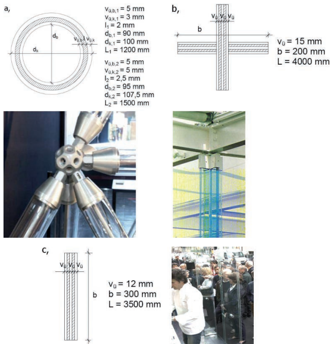
Fig. 2. Types of cross-sections [1, 6, 7]
