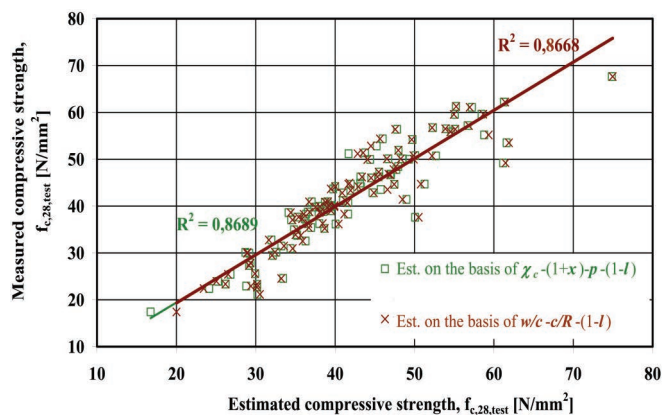
Fig. 11. Comparison of the errors of Eqs. (32) and (34) in estimating compressive strength
