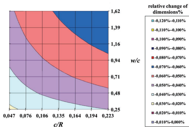
Fig. 23. Nomogram of deformation estimates based on w/c - c/R - \chi_c for mixes with CEM III/B 32.5 N-S at the age of t=112 days, when \chi_c=0.99 and f_2/f_1=183 (pure cement paste powder, medium sand content aggregate)
