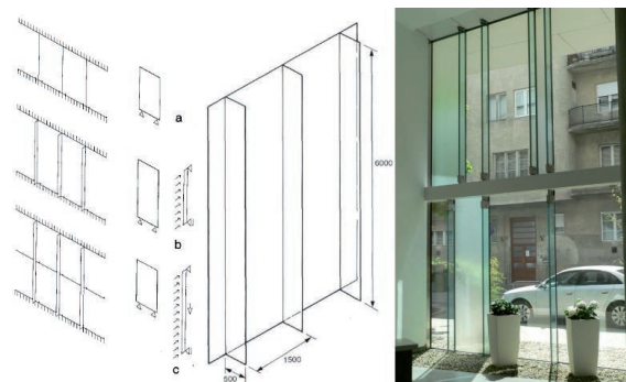
Fig. 3. Single and multi-storey glass columns [1, 5]; Budapest, Víziváros Business centre, Glass columns of Residence 1 building (structural design: Dr. Kinga Nehme)
