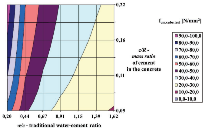
Fig. 15. w/c - c/R -(1- l )-based nomogram for mixes with stone powder and CEM I 42.5 N, based on experiments at ÉMI in 2010, ( l = 0.010 )
