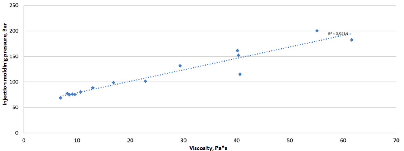
Fig. 4. The determined relationship between the capillary viscosity and injection molding pressure
