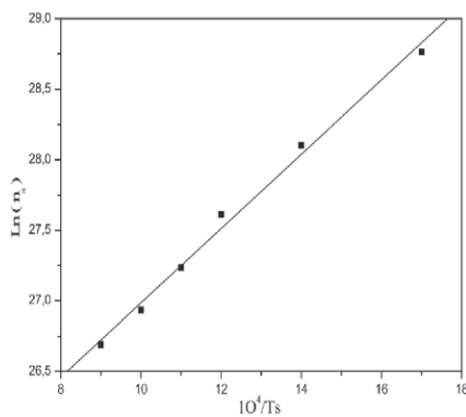
Fig. 2. Arrhenius plot of the saturation density of palladium clusters on MgO (100).
