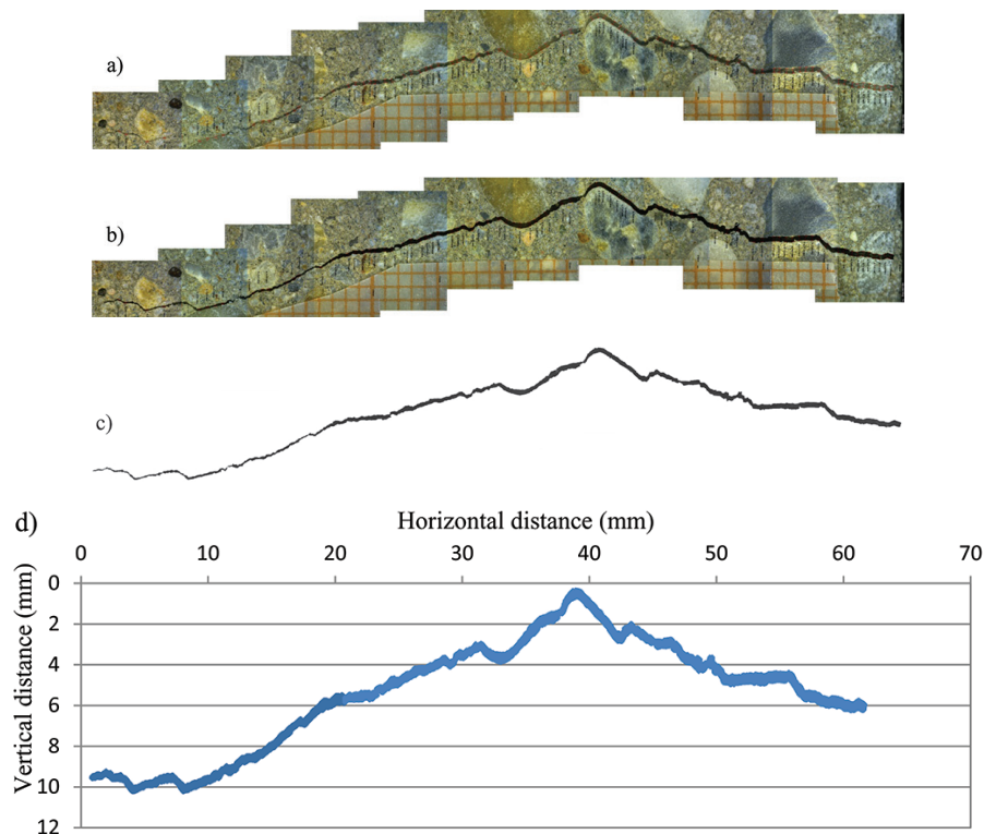
Fig. 1. Steps of digitalization a) original image b) crack after contrast adjustment c) separated crack d) crack drawn by pixel coordinates
