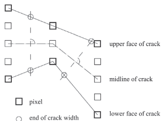
Fig. 2. Defining crack width - schematic diagram
