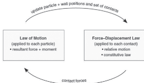
Fig. 1. Calculation cycle in PFC3D ( PFC3D User's Guide , 2008)
