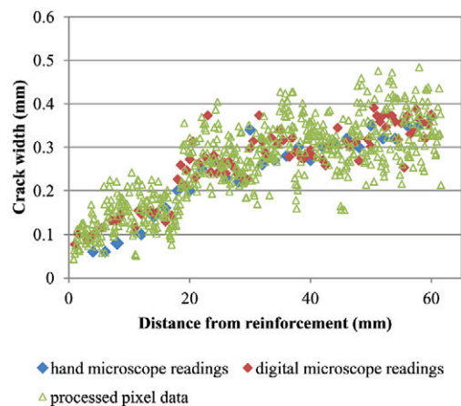
Fig. 4. Comparison of crack widths measured with hand microscope, digital microscope readings and image processing
