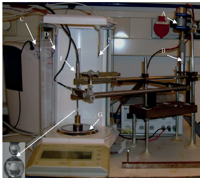
Fig. 3. Test device used for studying the interaction between two particles connected by a liquid bridge or two elements connected by a paste bridge. A: Velocity control armature, B: Micrometer screw, C: Humidifier, D: Temperature sensor, E: Humidity sensor, F: LVDT sensor, G: Scale.
