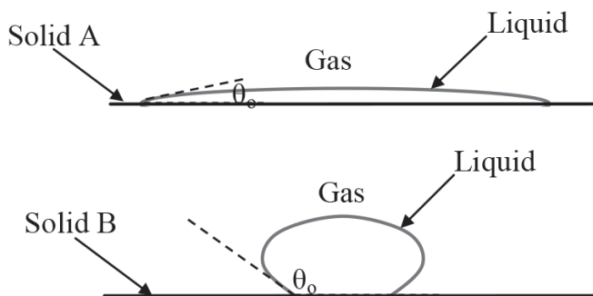
Fig. 2. Scheme of configuration of a liquid on a solid surface.
