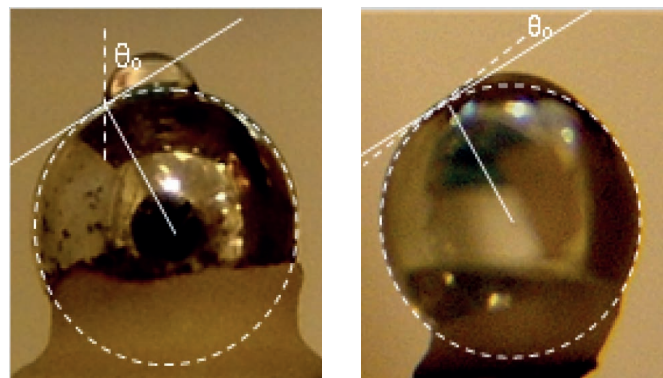
Fig. 4. Contact angle between a water drop and the surface of a particle.
