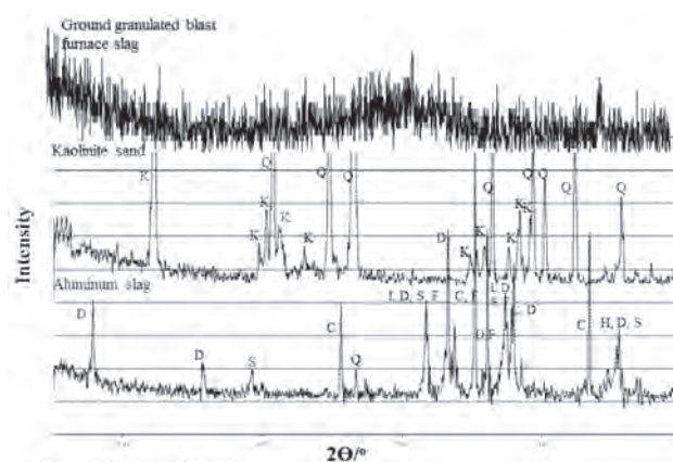
Fig. 1. X-Ray diffraction pattern of the starting raw materials [K=Kaolinite; Q=Quartz; D=Diaoyudaoite, syn ( \text{Na}_{1.22}\text{Al}_{11}\text{O}_{17.11} ); S=Spinel, syn ( \text{Mg}_{0.35}\text{Al}_{0.65}(\text{Al}_{1.78}\text{O}_4)_2 ); C=Corundum ( \text{Al}_2\text{O}_3 ); L=Lime ( \text{CaO} ); F=Fayalite magnesian ( \text{Mg}_{0.75}\text{Fe}_{1.10}\text{Mn}_{0.15}\text{SiO}_4 ); H=Halite ( \text{NaCl} )]
