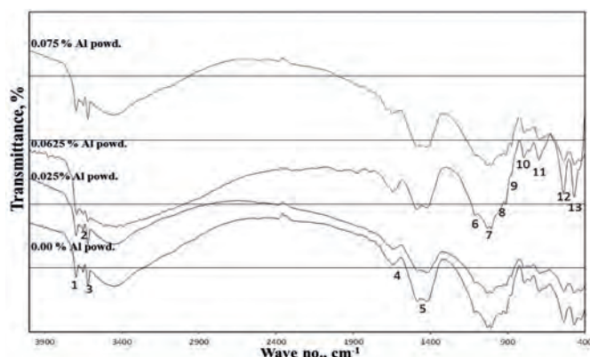
Fig. 3. FTIR spectra of 28 days lightweight geopolymer composite having various doses of aluminium powder [1,2,3: Stretching vibration of O-H bond for kaolin; 4: Bending vibrations of (HOH); 5: Stretching vibration of CO 2 ; 6: Asymmetric stretching vibration (Si-O-Si); 7: Asymmetric stretching vibration (T-O-Si); 8: Symmetric stretching vibration of Al-OH; 9: Symmetric stretching vibration of CO 2 ; 10: Symmetric stretching vibration (Al-O-Si); 11: Symmetric stretching vibration (Si-O-Si); 12,13: Bending vibration (Si-O-Si and O-Si-O)]
