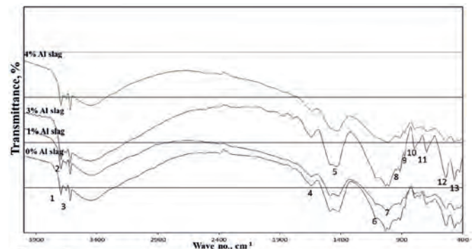
Fig. 8. FTIR spectra of 28 days lightweight geopolymer composite having various doses of aluminium slag [1,2,3: Stretching vibration of O-H bond for kaolin; 4: Bending vibrations of (HOH); 5: Stretching vibration of \text{CO}_2 ; 6: Asymmetric stretching vibration (Si-O-Si); 7: Asymmetric stretching vibration (T-O-Si); 8: Symmetric stretching vibration of Al-OH; 9: Symmetric stretching vibration of \text{CO}_2 ; 10: Symmetric stretching vibration (Al-O-Si); 11: Symmetric stretching vibration (Si-O-Si); 12, 13: Bending vibration (Si-O-Si and O-Si-O)]
