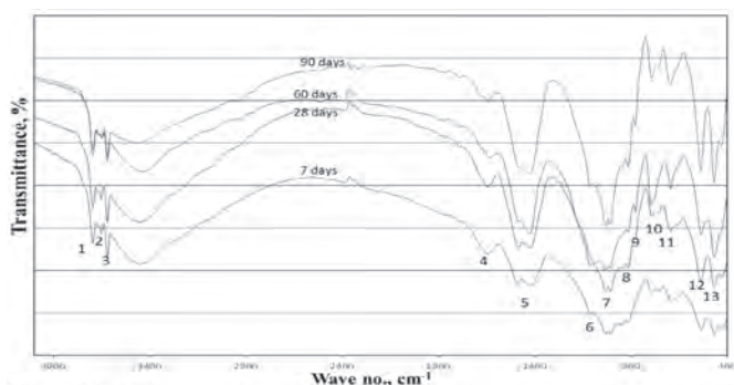
Fig. 2. FTIR spectra of control geopolymer cured up to 90 days in 40 °C with 100% R.H.) [1,2,3: Stretching vibration of O-H bond for kaolin; 4: Bending vibrations of (HOH); 5: Stretching vibration of CO 2 ; 6: Asymmetric stretching vibration (Si-O-Si); 7: Asymmetric stretching vibration (T-O-Si); 8: Symmetric stretching vibration of Al-OH; 9: Symmetric stretching vibration of CO 2 ; 10: Symmetric stretching vibration (Al-O-Si); 11: Symmetric stretching vibration (Si-O-Si); 12,13: Bending vibration (Si-O-Si and O-Si-O)]
