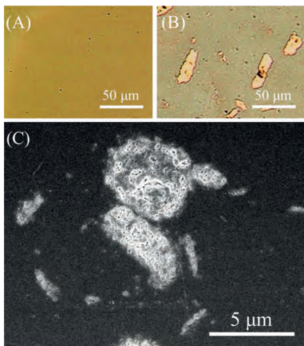
Fig. 4 Optical images on the polished surface of the sintered bodies for (a) monolithic \text{Si}_3\text{N}_4 (SN_25) and (b) Ti-added \text{Si}_3\text{N}_4 (SNTi_25), and SEM image on the surface for (c) Ti-added \text{Si}_3\text{N}_4 (SNTi_40)
