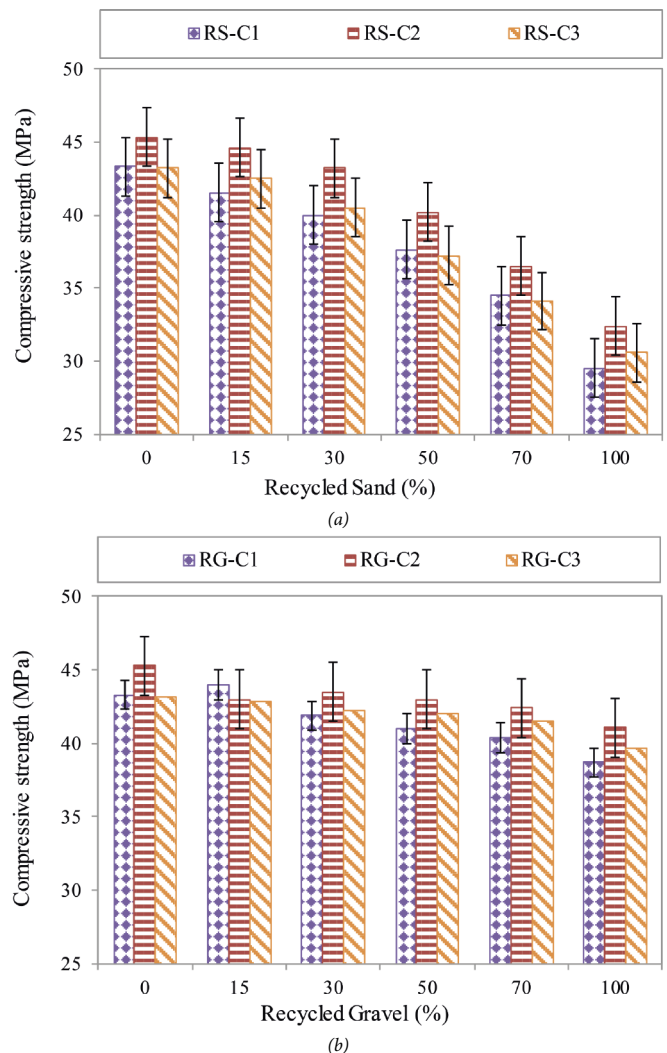
Fig. 12 Compressive strength evolution of RAC with three cement / admixture and with RA substitution rate at 28 days: (a) RS; (b) RG
