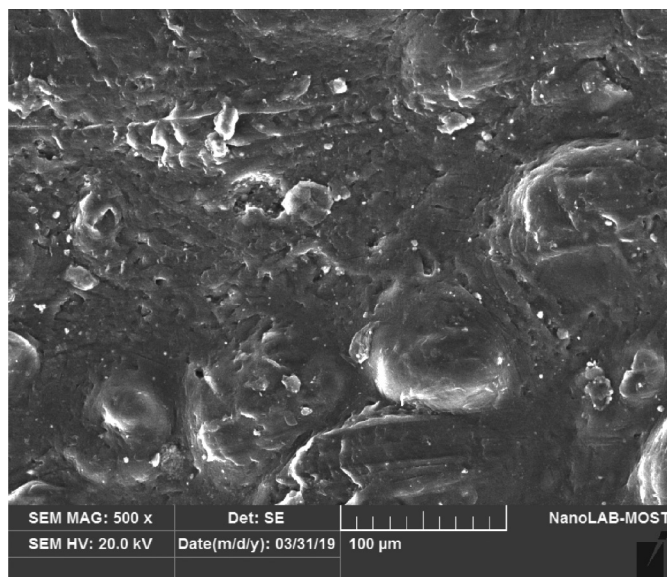
Fig. 15 SEM of polymer modified with CNT
