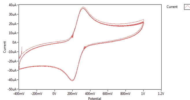
Fig. 18 Cyclic voltammogram of 0.1M K_4[Fe(CN)_6] in 0.1M KCl at ten times using polymer working electrode modified with CNT
