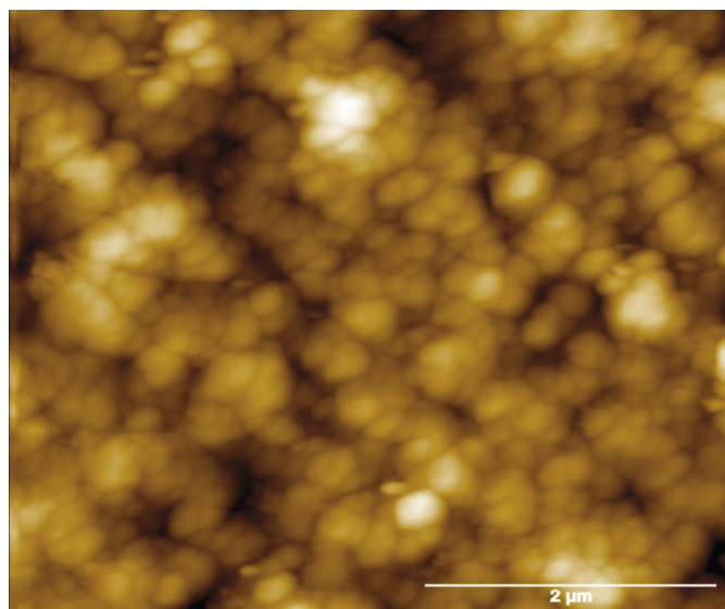
Fig. 16 AFM of the polymer modified with CNT
