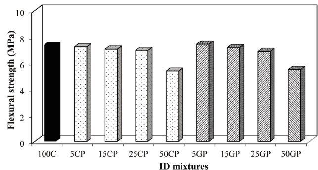
Fig. 8 Flexural strength for mortar mixtures with plain and blended cements at 28 days
