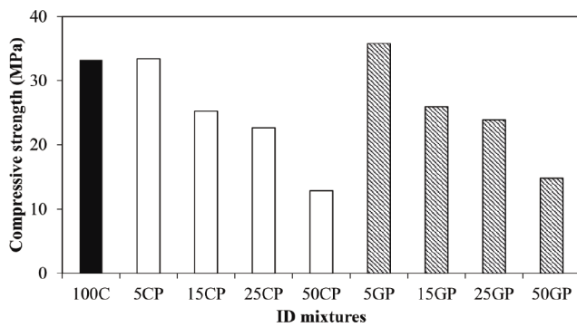
Fig. 4 Compressive strength for mortar mixtures with plain and blended cements at 3 days
