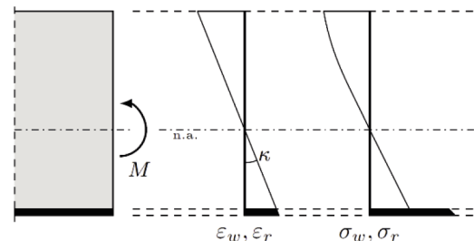
Fig. 2 Axial stresses and strains in the Euler beam.
