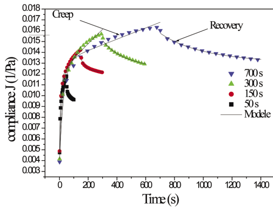
Fig. 1 Evolution of the elastic compliance of the slip as a function of time for different time applied
