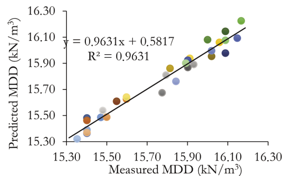
Fig. 1 Predicted MDD versus measured MDD values for the various Li-IOT-BCS mixtures
