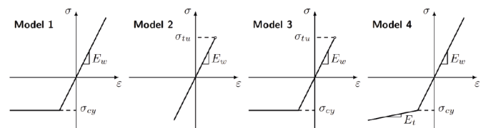
Fig. 4 Stress-strain curves for four different wood models.
