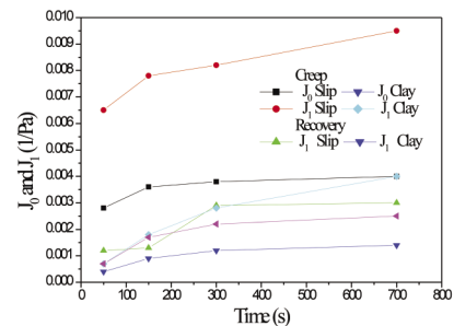
Fig. 3 Variation of the instantaneous elastic compliance J_0 and delayed J_1 of the Nedroma clay and slip of ceramic as a function of applied time
