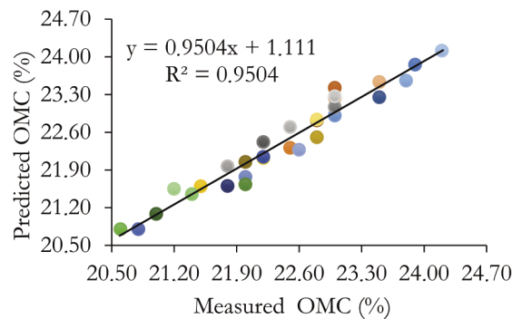
Fig. 2 Predicted OMC versus measured OMC values for the various Li-IOT-BCS mixtures
