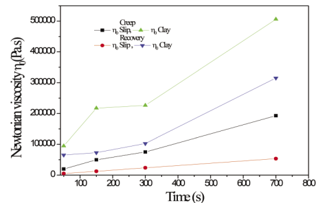
Fig. 4 Variation of Newtonian viscosity of the slip and the Nedroma clay as a function of applied time
