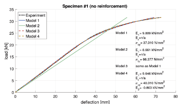
Fig. 5 Measured and simulated load-deflection curves for specimen 1.
