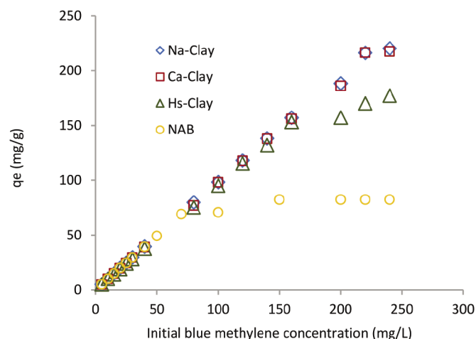
Fig. 5 Isotherms of MB adsorption onto NAB, Na-Clay, Ca-Clay and Hs-Clay adsorbents
