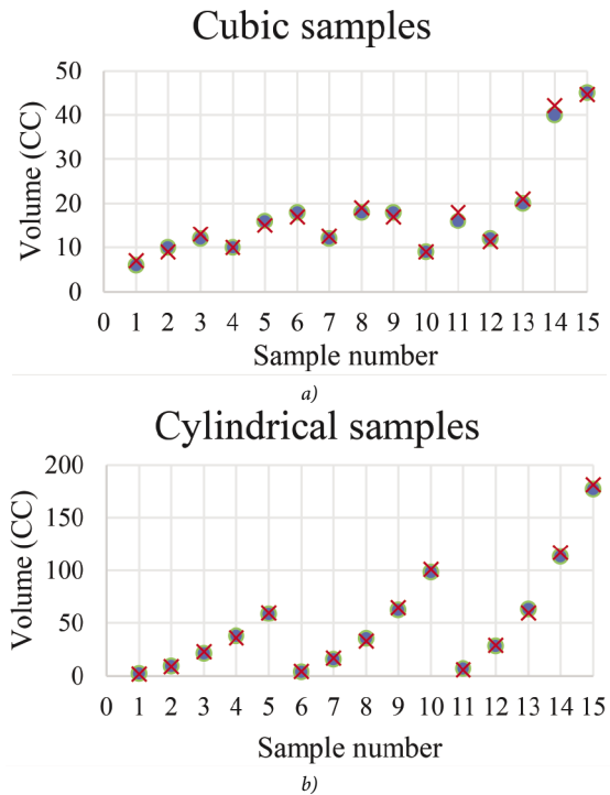
Fig. 3 The difference in obtained volume from geometrical measurement and modified Archimedes measurement in cubic (a) and cylindrical samples (b) (the red marks show data for geometrical volume and the blue marks represent the Archimedes measurements)
