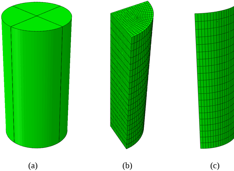
Figure 3 Geometric representation of FE model: (a) full specimen, (b) mesh of 1/4 concrete specimen, and (c) mesh of 1/4 FRP jacket.
