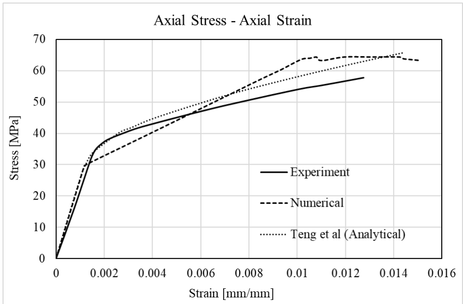
Figure 4 stress strain curve for experimental and numerical
