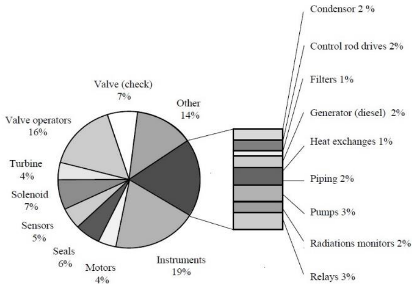
Figure 5. Distribution of valve failures on the various subsystems of boiling water nuclear power plants [15]
