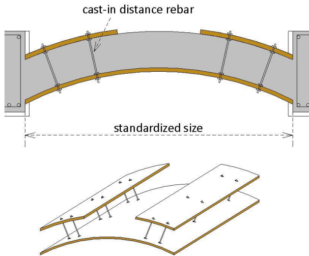
Figure 14.: The required framework for constructioning the beams and the vaults between them (author's drawing)
