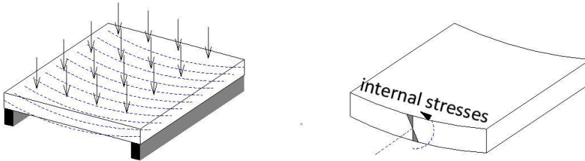
Figure 9.: Typical bent floor slab structures ( author's drawings )
