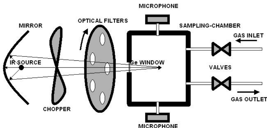
Figure 5 The set-up of the Photoacoustic Spectrometer
