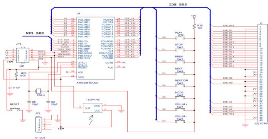
Figure 1 Microcontroller connections
