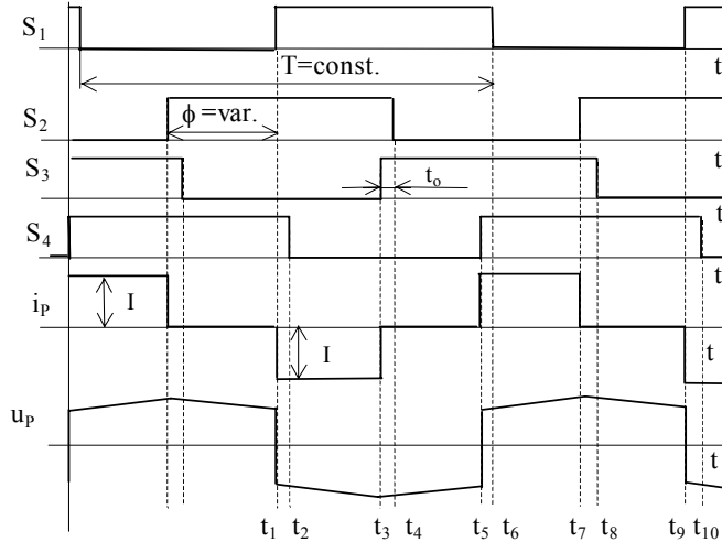
Figure 13 Idealised waveforms of the FB ZCS PWM converter
