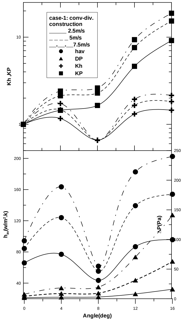
Figure 6a Variation of performance against \beta for case 1 (convergent – divergent)
