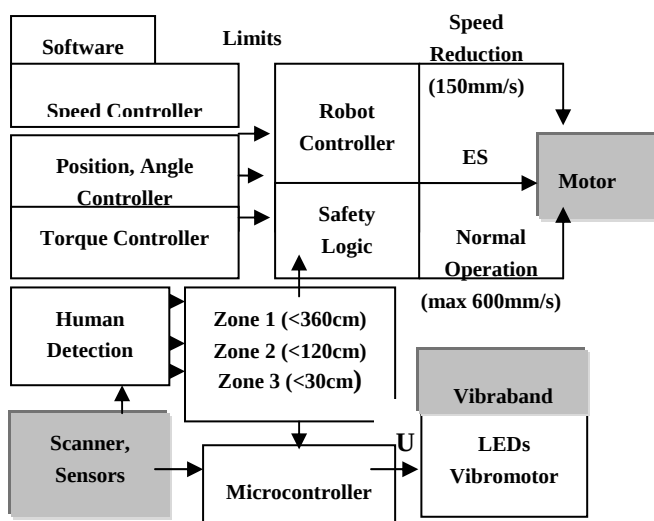
Figure 6 Control Algorithm
