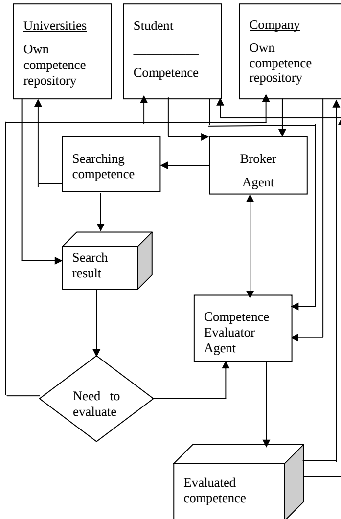
Figure 1 The multi-agent system for the proposed model
