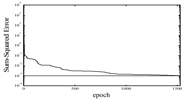
Figure 14 Training error
