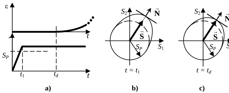
Figure 10 Creep delay
