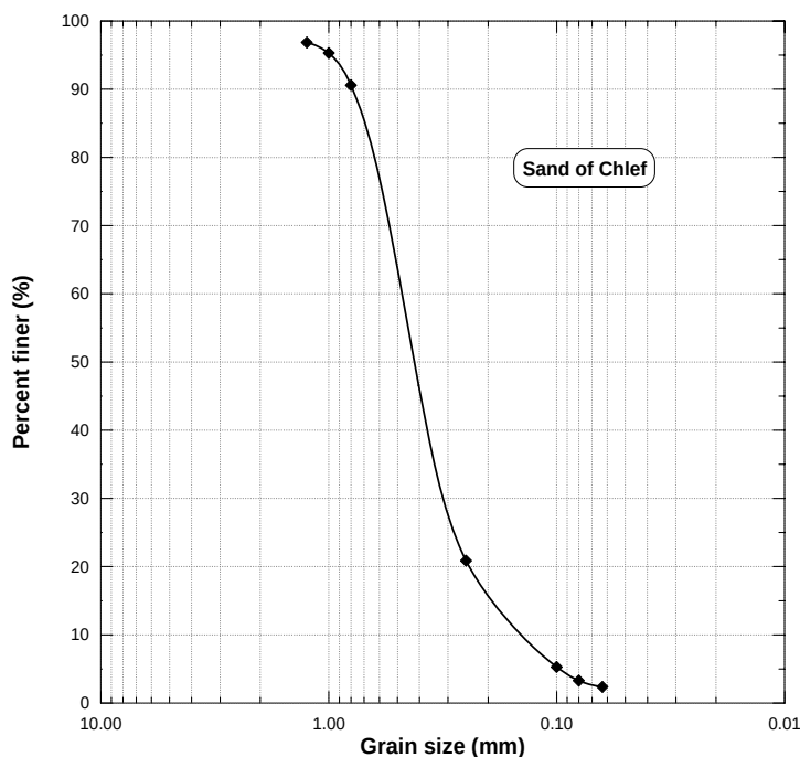
Figure 5 Grain size distribution of the tested soil
