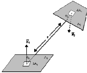
Figure 4 Form-factor geometry
