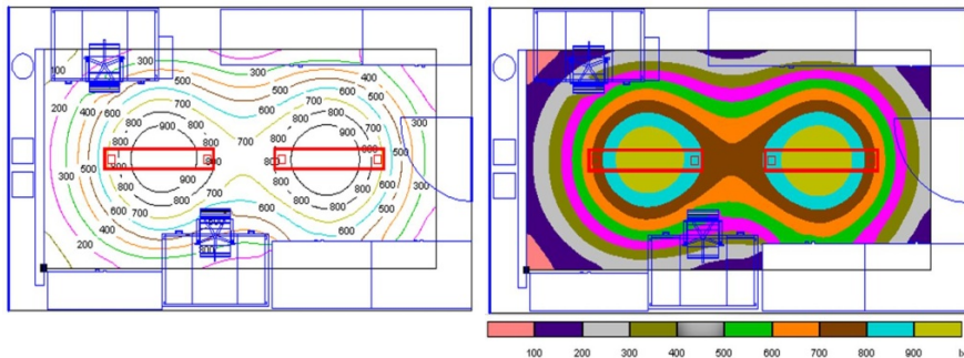
Figure 6 Isofotoc lines
