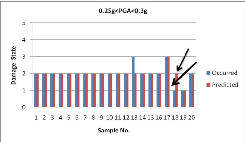
Figure 6 Comparison of ANN prediction to actual damage state for 0.25 g <PGA<0.3 g
