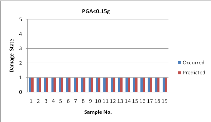
Figure 5 Comparison of ANN prediction to actual damage state for PGA<0.15 g
