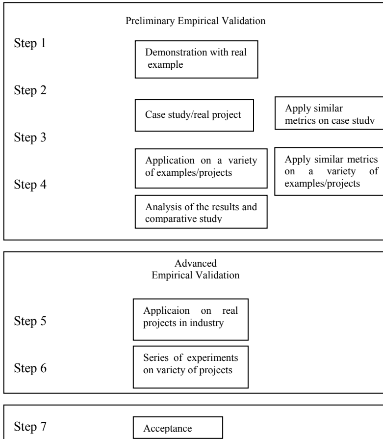
Figure 1 Proposed Model for Empirical Validation of Software
