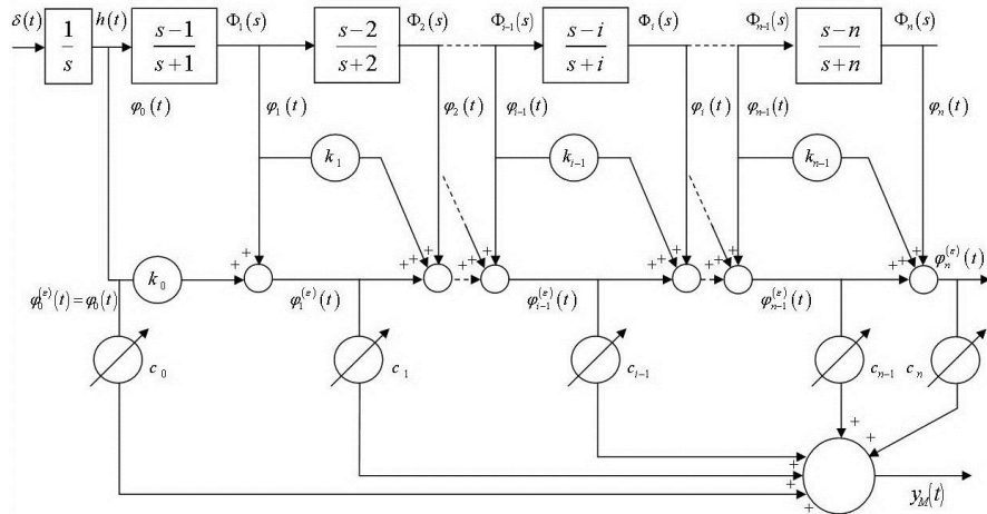
Figure 1 Adjustable model of imperfect system
