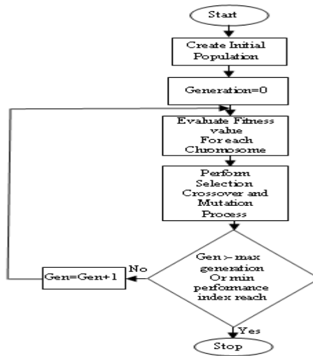
Figure 3 Genetic Algorithm Architecture
