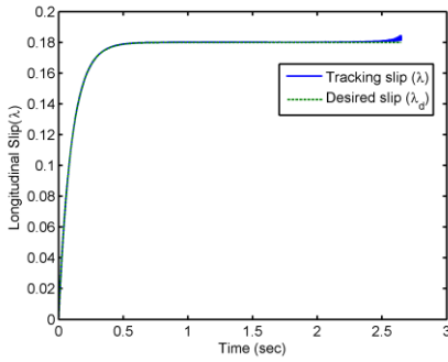
Figure 8 Slip tracking using FBL with \mu = 0.85
