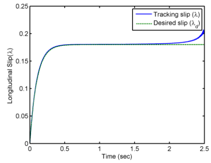
Figure 9 Slip tracking using FBLPID with \mu = 0.85
