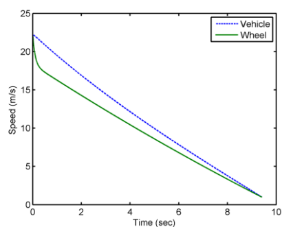
Figure 7 Vehicle & wheel deceleration using FBLPID controller with \mu = 0.2
