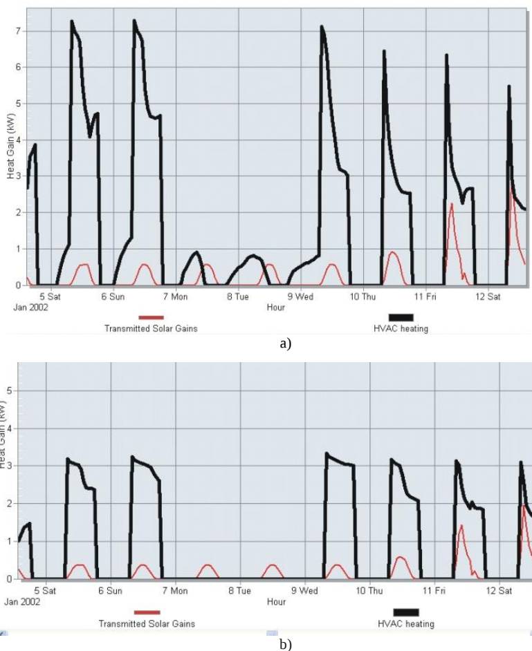
Figure 8 DesignBuilder simulation results for classroom HVAC heating and solar gains: a) Old window; b) New window
