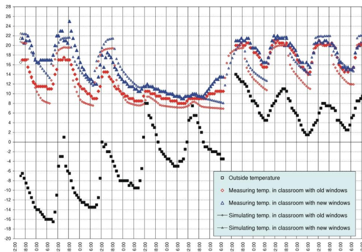
Figure 6 Simulated and measured indoor and outdoor air temperatures
