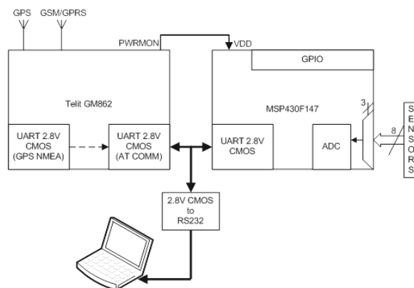
Figure 1 The structure of GPRS microcontroller system
