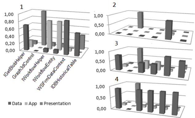
Figure 4 Unit rate assignments (1-by name; 2-by base types; 3-by namespace; 4-by project)
