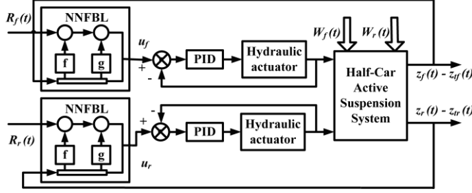
Figure 3 Control architecture
