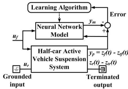
Figure 4 System identification of the half-car AVSS for NNFB control
