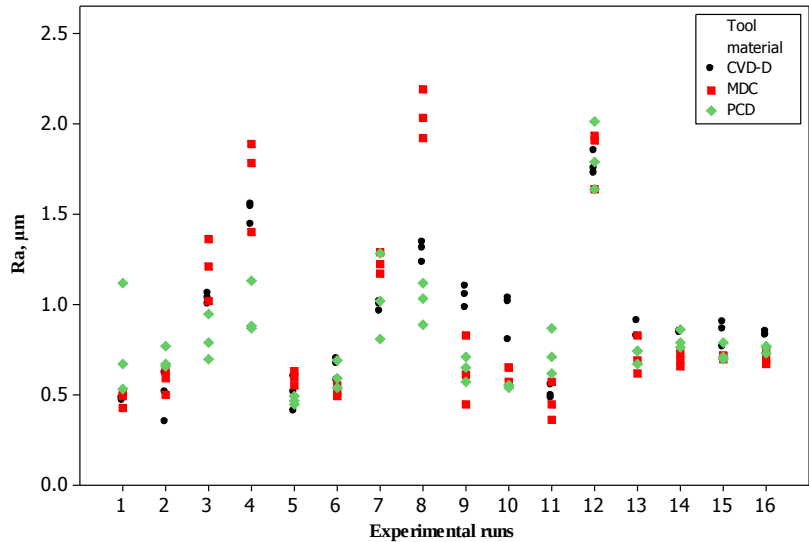
Figure 1 The values of average surface roughness ( Ra ) obtained by the examined tools
