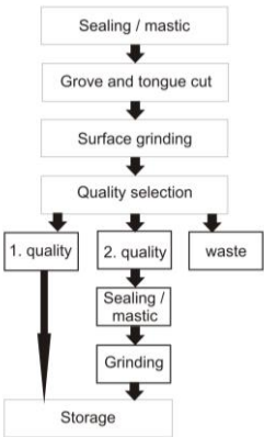
Figure 6 Fifth sub-process – Machine processing
