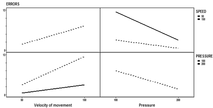
Figure 13 Interaction of factors measured on Response
