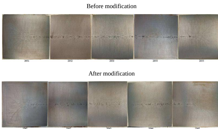
Figure 10 Macroetched cross sections of slabs cast with the original (above) and modified (bottom) roll setting (thickness of slab: 240 mm)
