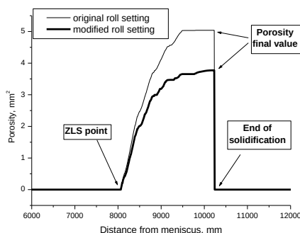
Figure 9 Expected porosity in casting case No. 136
