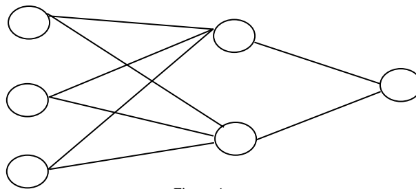
Figure 4 Neural Network
