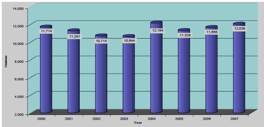
Figure 9 RTA 2000 – 2007
