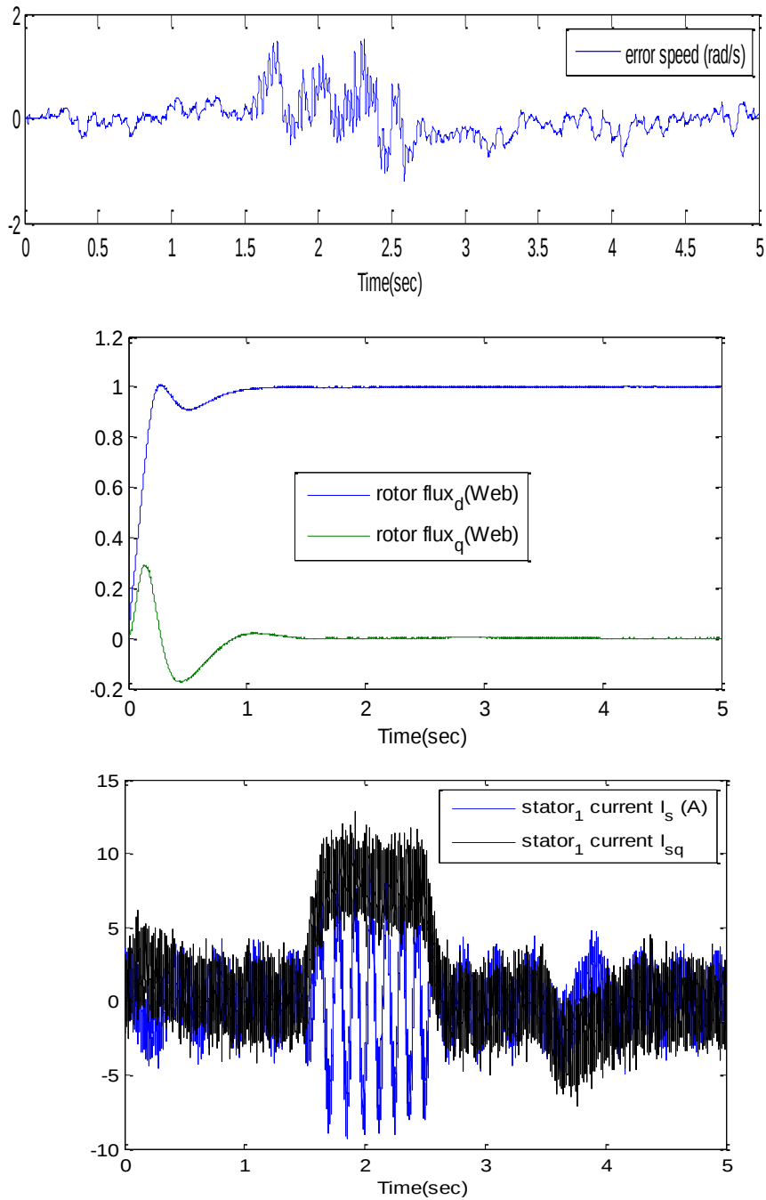
Figure 9 Error speed ,rotor flux and stator current results for low speed sensorless control
