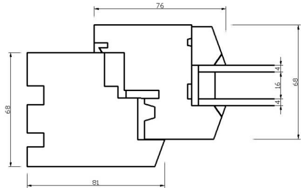
Figure 3 Horizontal section of the window studied (sizes in mm)
