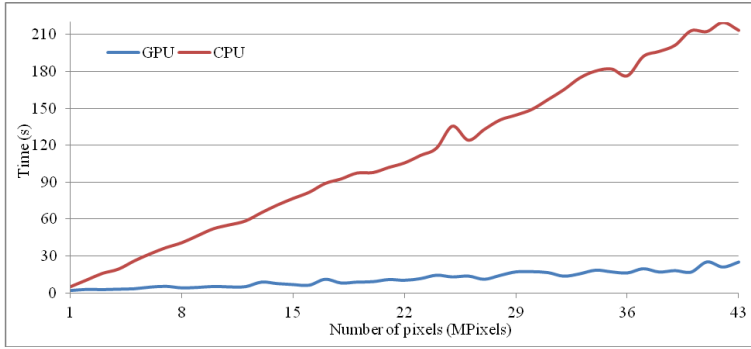
Figure 6 GPU vs. CPU execution across the entire test domain
