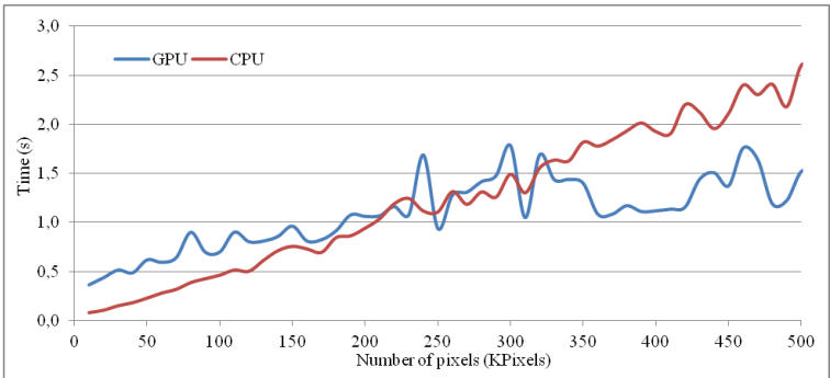
Figure 5 GPU vs. CPU execution for small workloads
