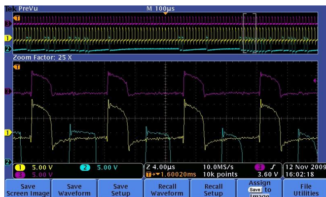
Figure 14 Examination of BITS signals
