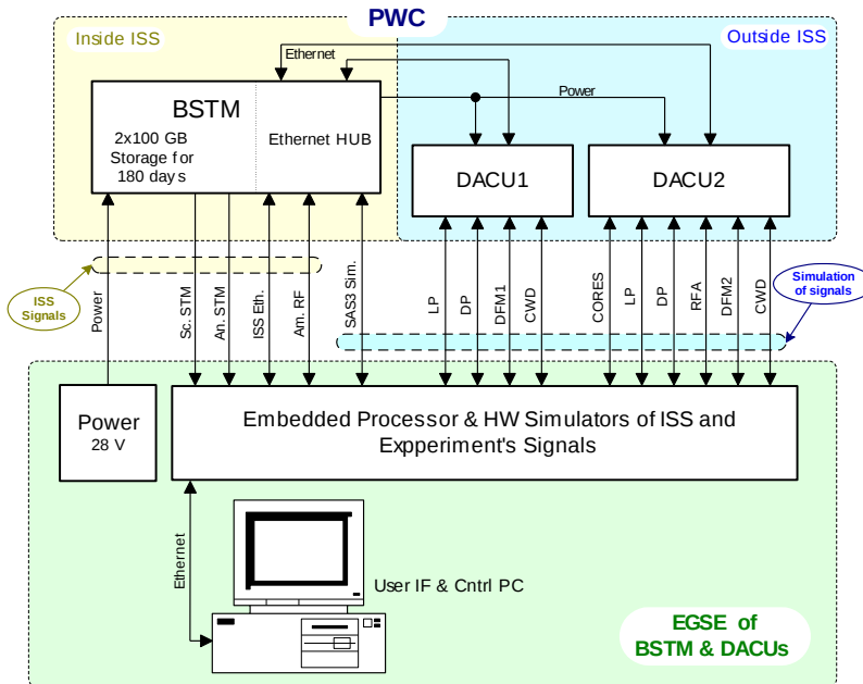
Figure 10 Test arrangement of Obstanovka computers with EGSE during test
