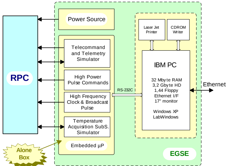
Figure 5 The Blockscheme of TEGSE for the RPC instrument for Rosetta
