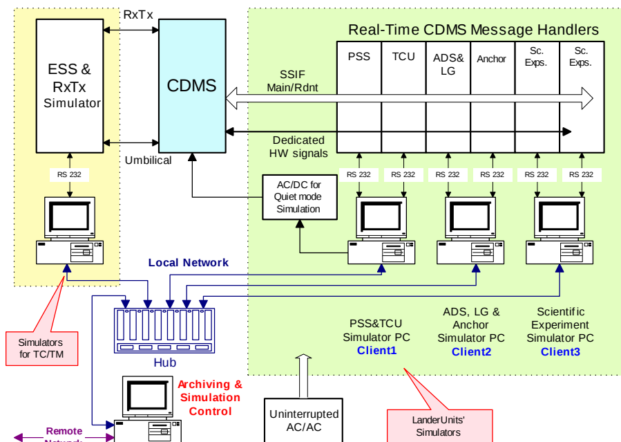
Figure 8 Blockscheme of test environment of CDMS
