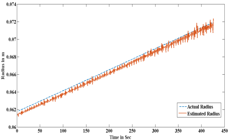
Figure 6 Comparison between actual winder radius and the online estimated radius
