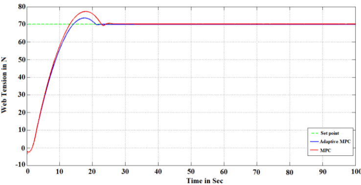
Figure 7 Responses of Adaptive MPC and MPC to a reference web tension of 70 N
