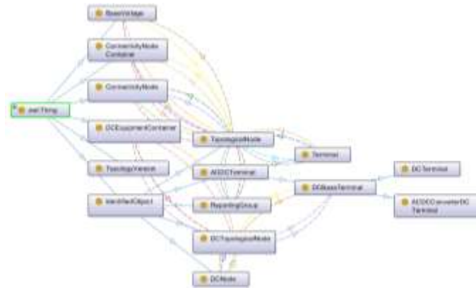
Figure 1 OntoGraph Vizualization of Topology Profile Ontology in Protégé
