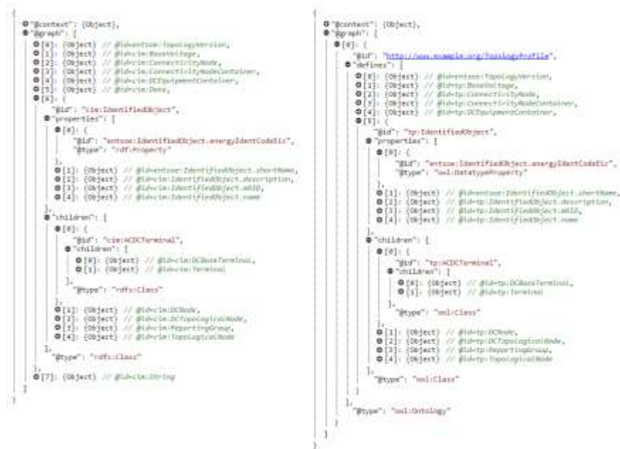
Figure 2 JSON Tree View of TopologyProfile in RDFS (left) and OWL 2 (right)
