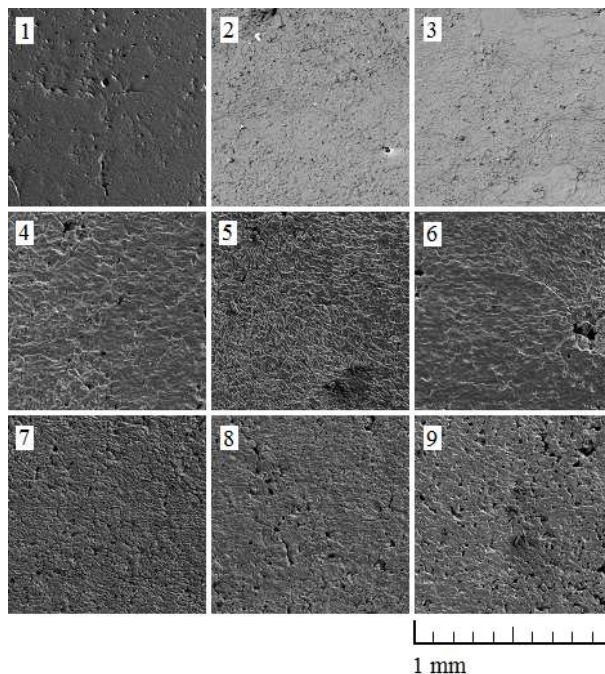
Figure 9 Microstructure in specific areas No. 1–9 of the thin plate surface ( \times 166 )
