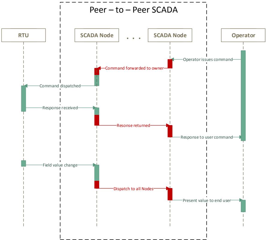
Figure 4 Sequence diagram of basic SCADA operations
