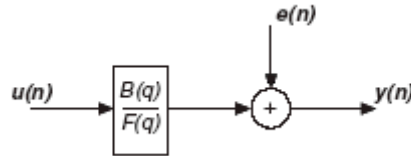
Figure 4 Output - Error model architecture [29]
