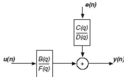
Figure 5 The structure of the Box - Jenkins model [29]
