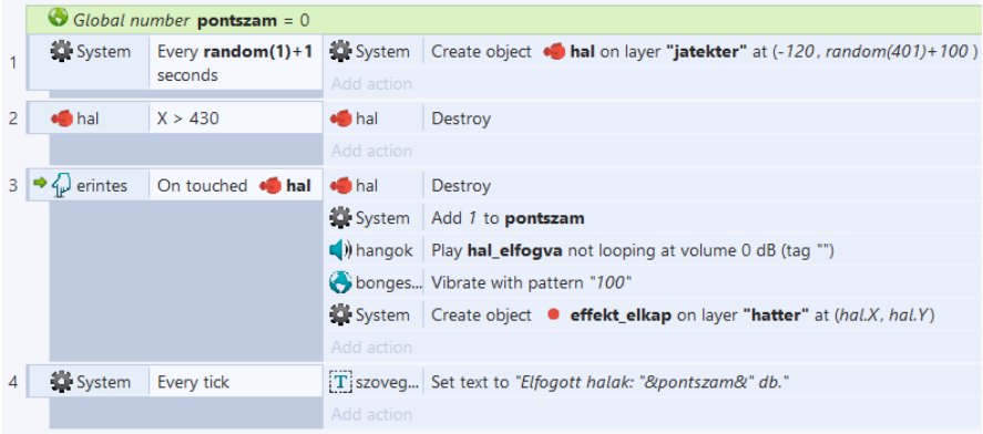
Figure 2 The visual source code of the core functionalities of the workshop project
