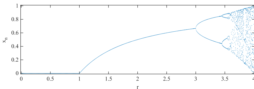
Figure 1 A bifurcation diagram of the logistic map
